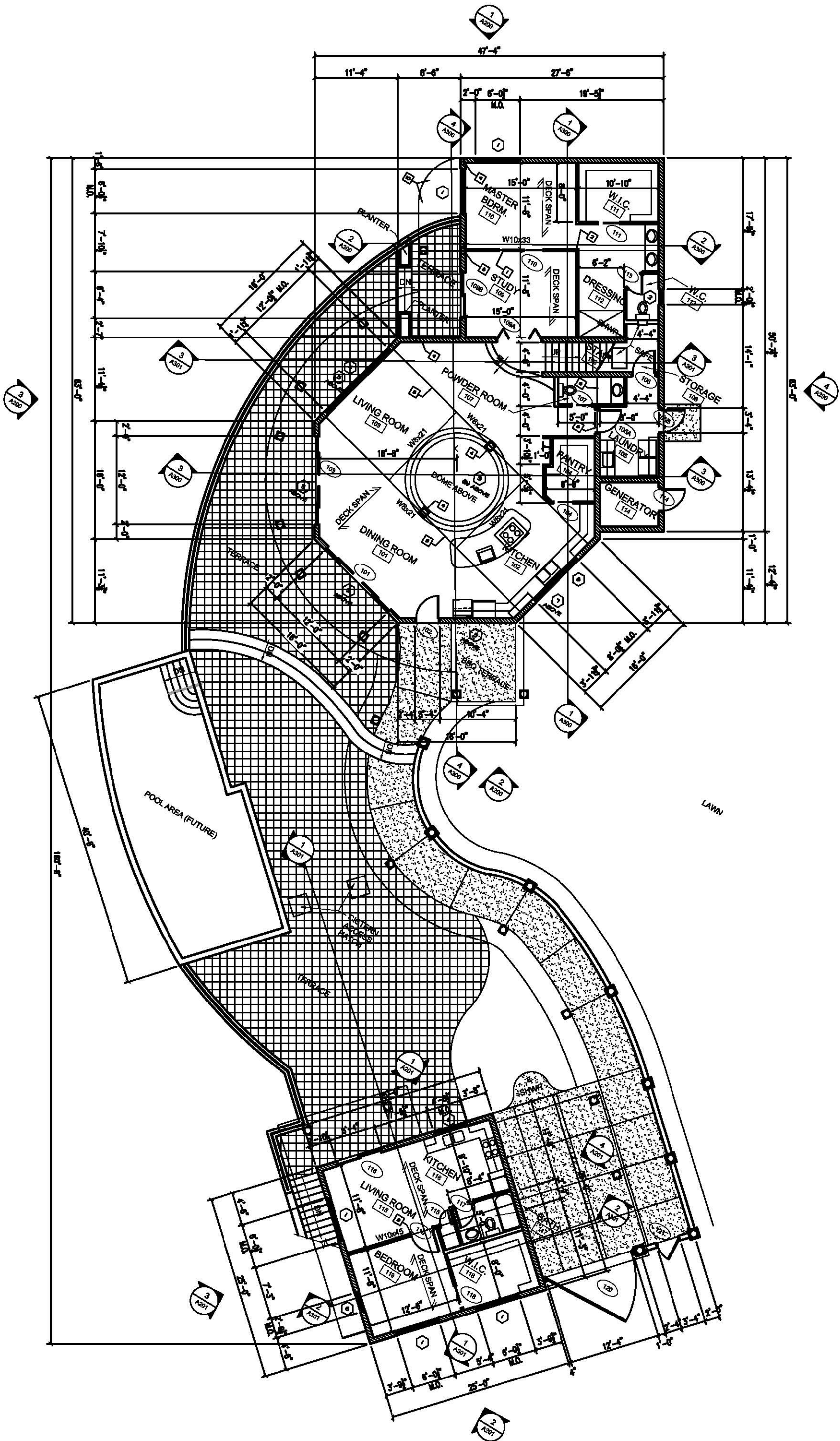
1 MAIN LEVEL FLOOR PLAN SCALE: 1/8"=1'-0"
